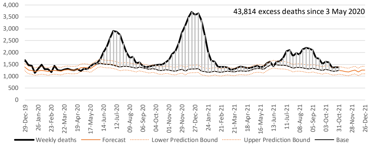
Eastern Cape weekly deaths from natural causes : 29 Dec 2019 - 6 Nov 2021
