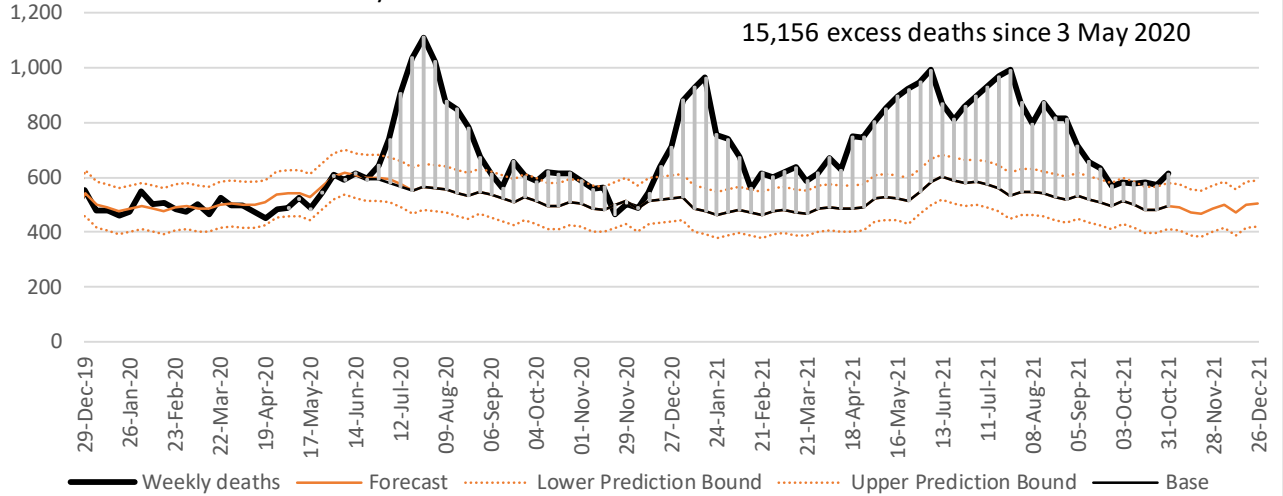
Free State weekly deaths from natural causes : 29 Dec 2019 - 6 Nov 2021
