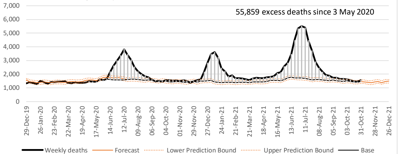
Gauteng weekly deaths from natural causes : 29 Dec 2019 - 6 Nov 2021
